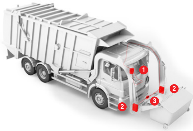
1 Weighing electronics
