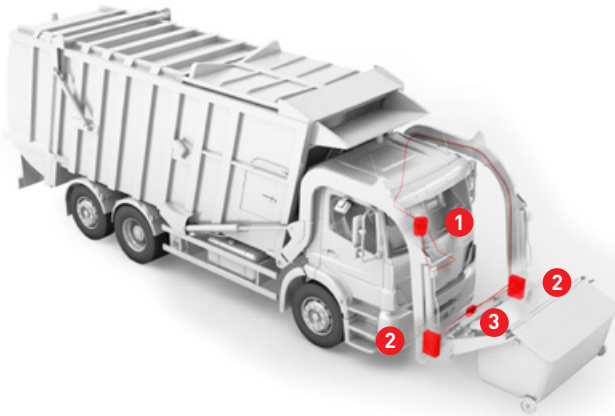
1 Weighing electronics
